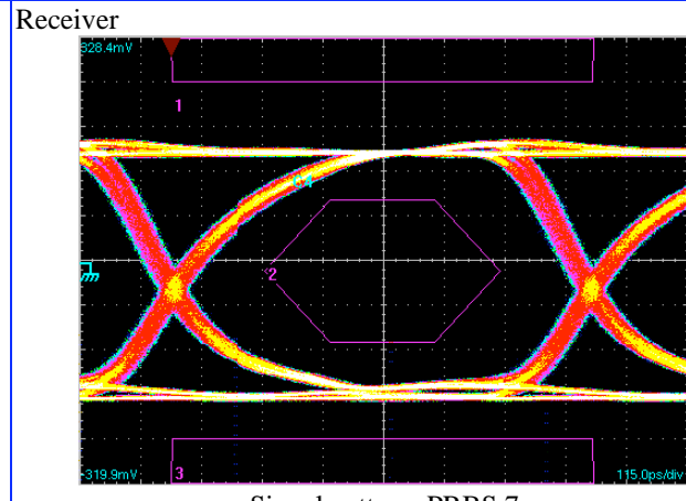
Signal pattern: PRBS 7 Input Power: -19 dBm
