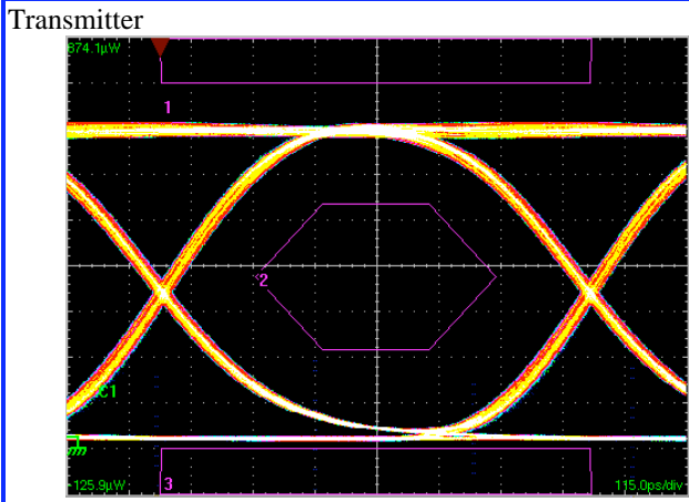
Signal pattern: PRBS 7
