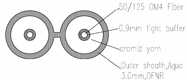
∅3.0mm OFNR cable section
